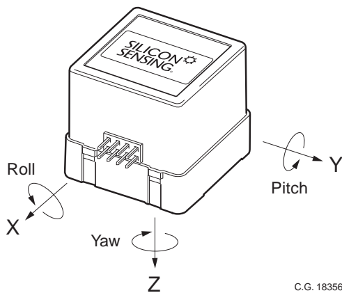
Figure 1 Co-ordinate Set for the DMU02 System
