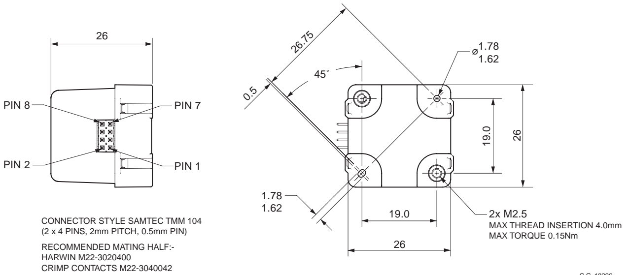
Figure 2 DMU02 Physical Outline
