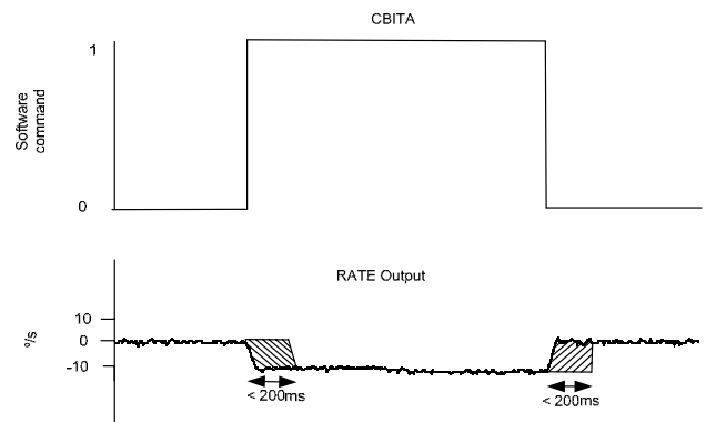
Figure 8 CBITA Timing
